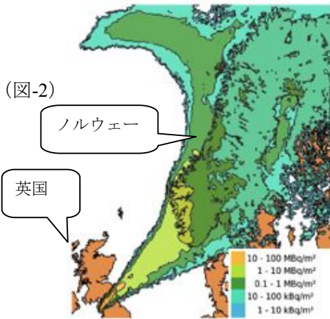
Figur 4.3: Fallout of ^{137}\text{Cs} ( \text{Bq}/\text{m}^2 ) after a worst case accident releasing 10% of the total assumed ^{137}\text{Cs} inventory from the HASTs at Sellafield.
